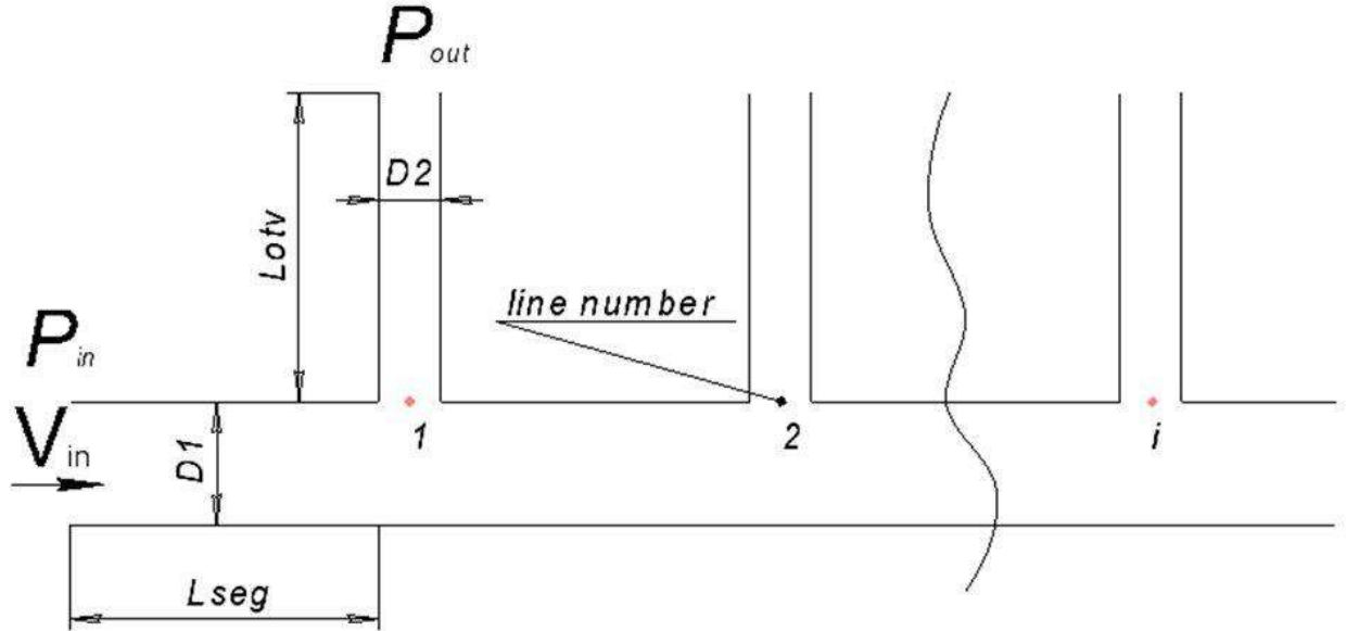
Fig. 1 – Schematic Diagram of the Main Pipeline.
