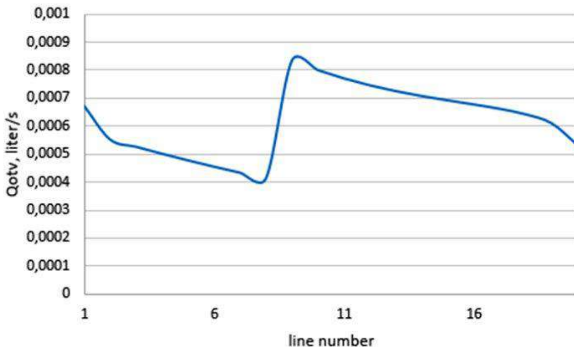
Fig. 3 – Flow Rate Variation vs. Branch Number After Section Optimization.
