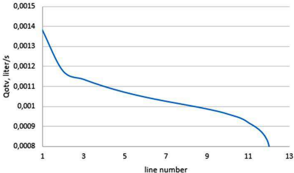
Fig. 2 – Flow Rate Variation vs. Intake Branch Number
